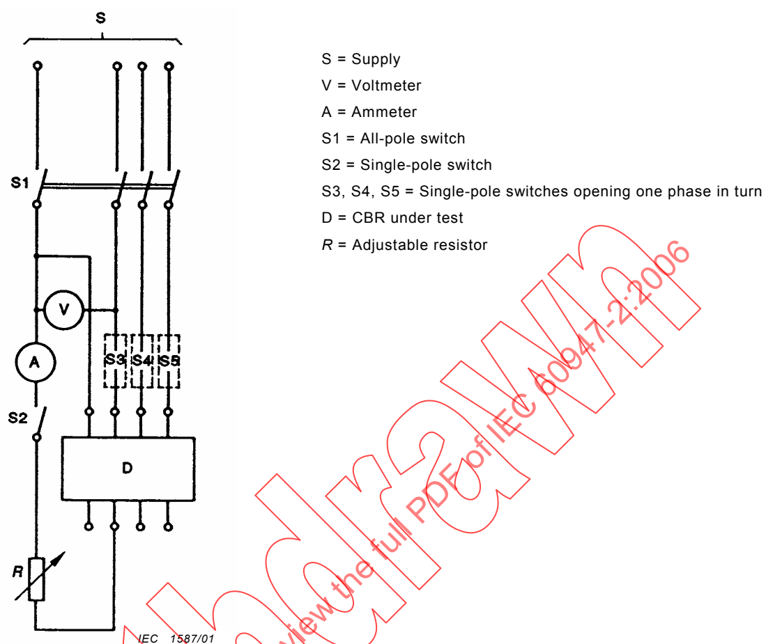
Figure B.3 – Test circuit for the verification of the behaviour of CBRs classified under B.3.1.2.2 (see B.8.9)
