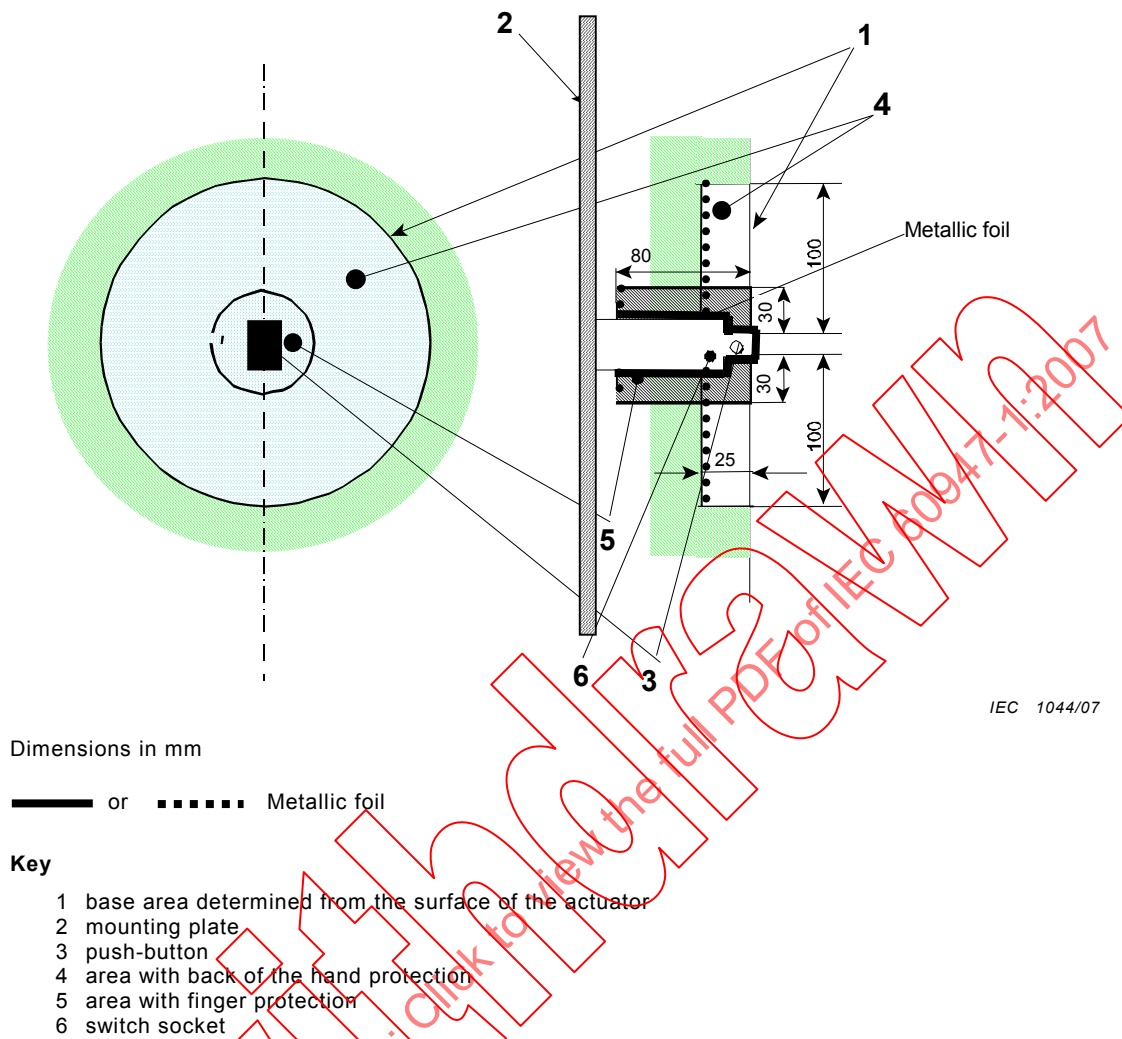
Figure R.2 – Operating space for push-button actuation
