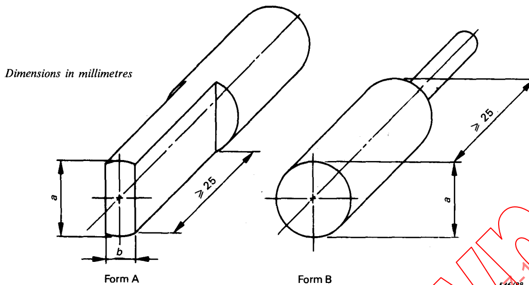
FIG. 2. — Gauges of form A and form B.
