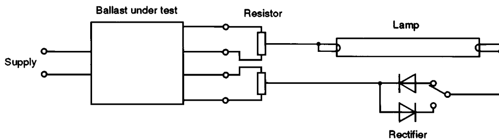
Figure 1 – Circuit for testing rectifying effect
