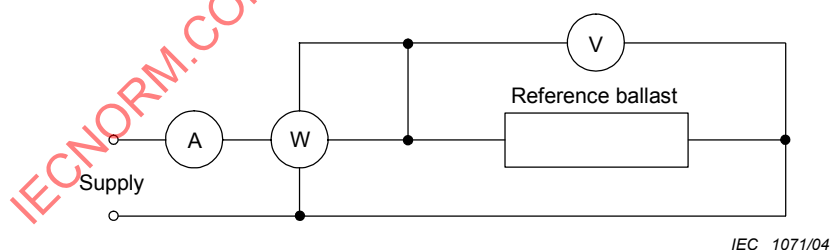
Figure A.2 – Recommended circuit for the determination of power-factor of the reference ballast
