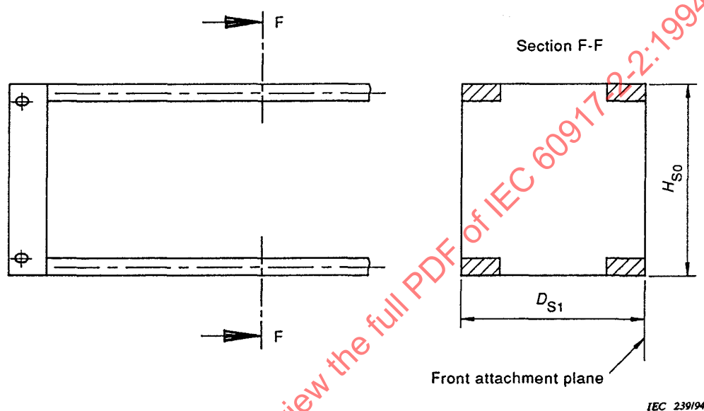
Figure 6 – Type C subrack dimensions
