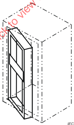
Figure 6 – Cadre oscillant
