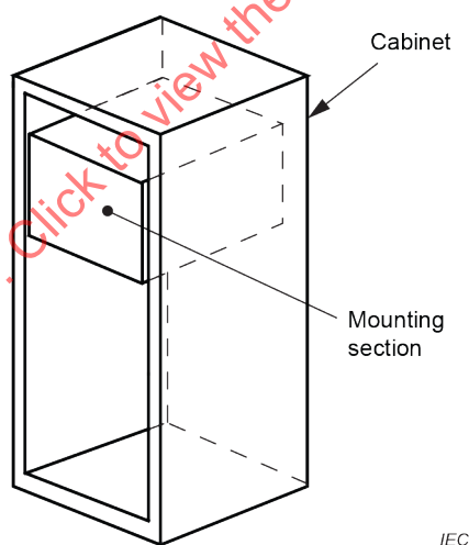
Figure 20 – Mounting section
