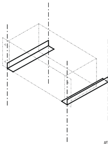
Figure 12 – Glissières
