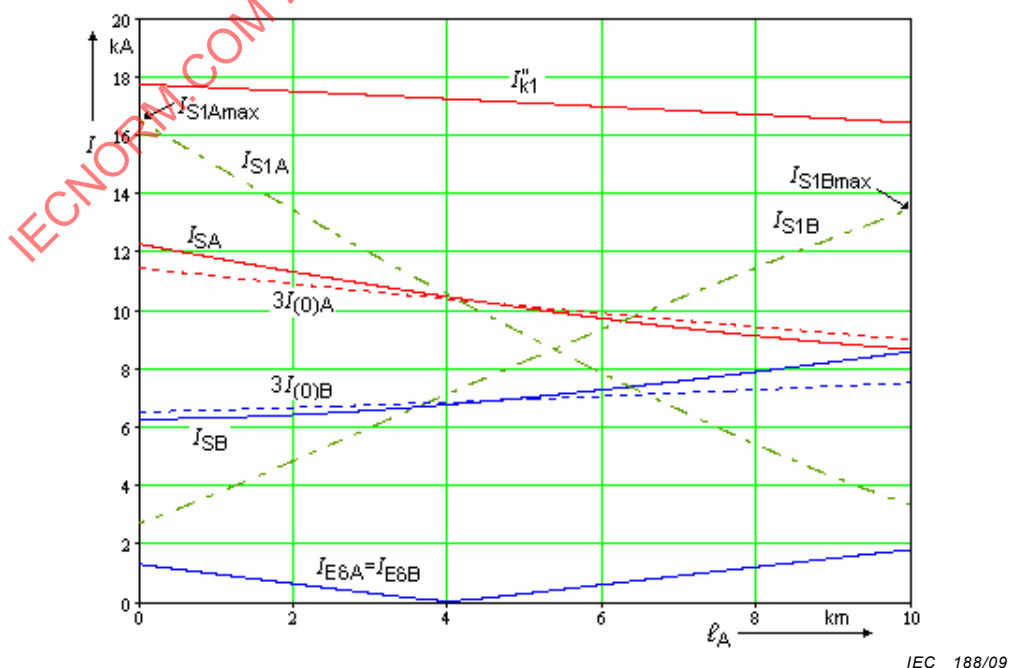
Figure D.6 – Current distribution for the cable in Figure D.4 depending on \ell_A , R_{EF} \rightarrow \infty
