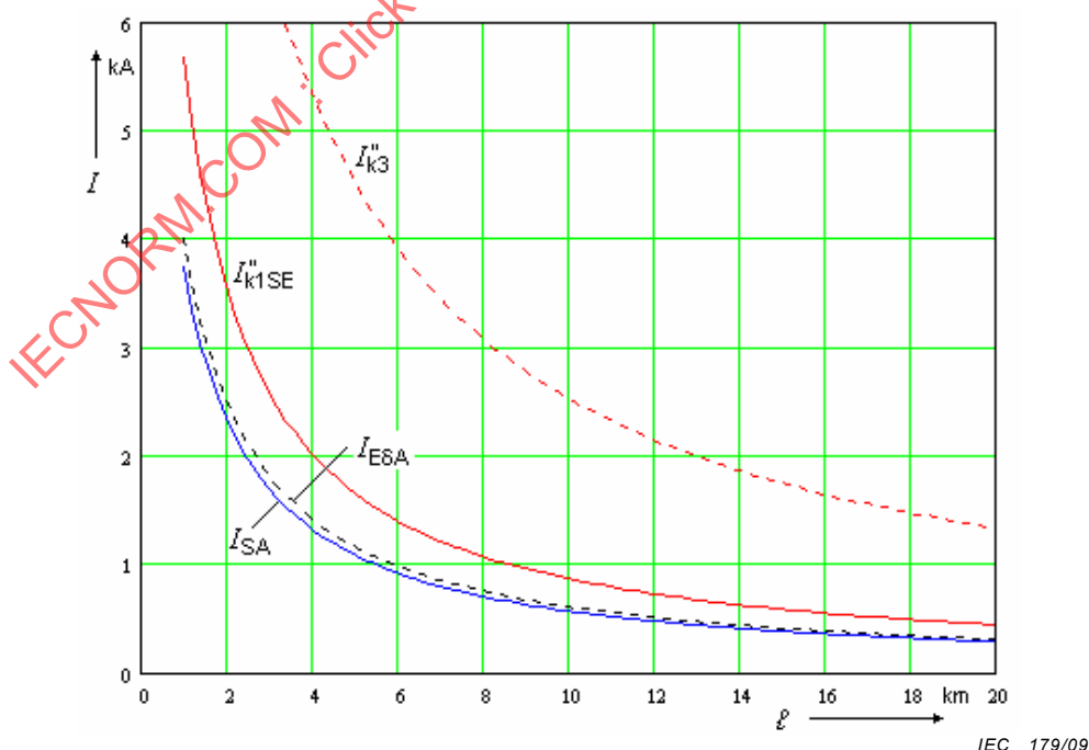
Figure C.2 – Short-circuit currents and partial short-circuit currents through earth for the example in Figure C.1
