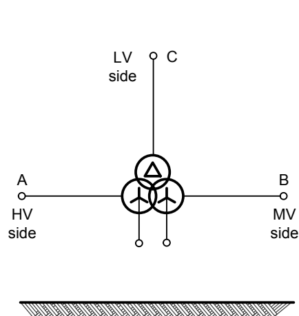
Figure 6a – Denotation of winding connections
