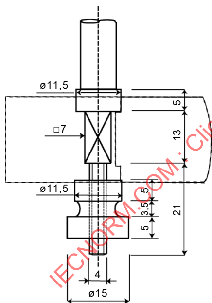
Detail of the assembly of hammer
