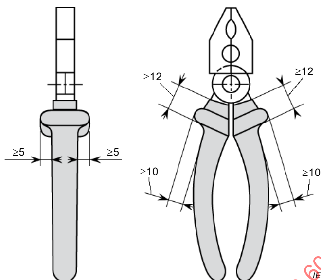
Figure 8 – Insulation of pliers
