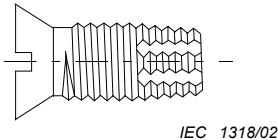
Figure 7 – Example of thread-cutting screw
