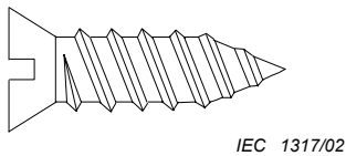
Figure 6 – Example of thread-forming screw
