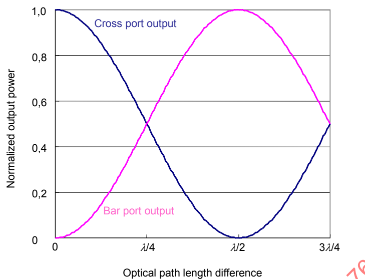
Figure D.2 – Output power of TO switch
