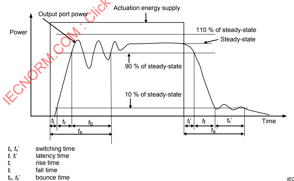
Figure 1a – Non-latching switch, normally off
