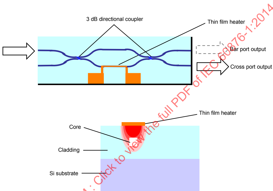
Figure D.1 – Example of TO switch
