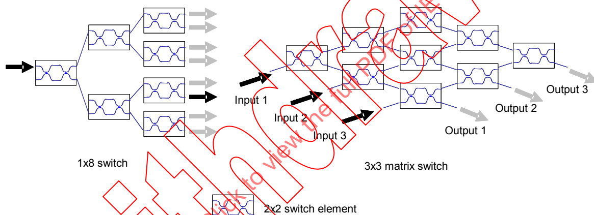
Figure A.8 – 1 \times N and N \times N examples of TO switch
