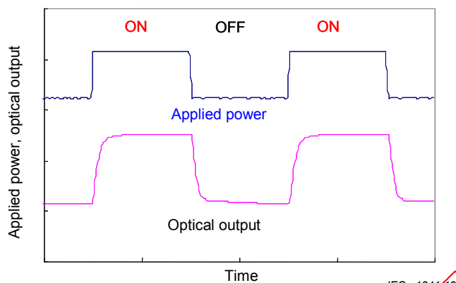
Figure A.7 – Example of switching response of TO switch
