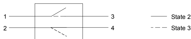
Figure 8 – Four-port switch without crossover
