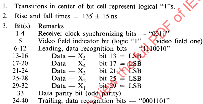
FIG. 13. — 40-bit system, bit cell length and digital level (Sub-clause 10.2).
