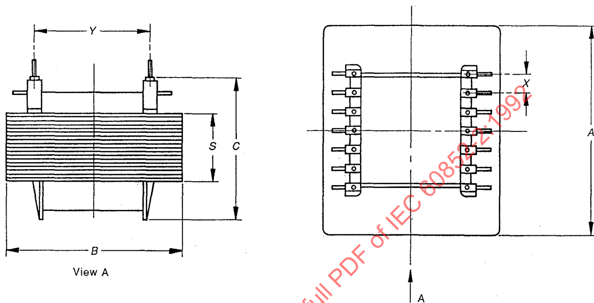
Figure 1 – PWB mounting style for laminations YEx 2-2 to YEx 2-12: standard configuration
