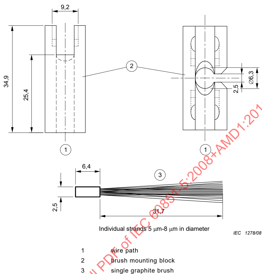
Figure 8a – Graphite fibre single brush electrode assembly
