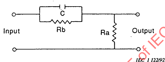
Figure 3 – Main pre-emphasis circuit
