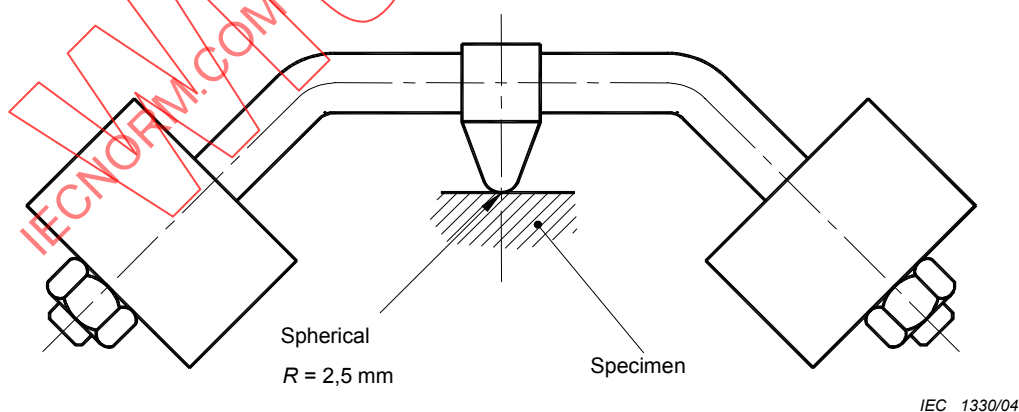
Figure 1 – Ball-pressure test apparatus
