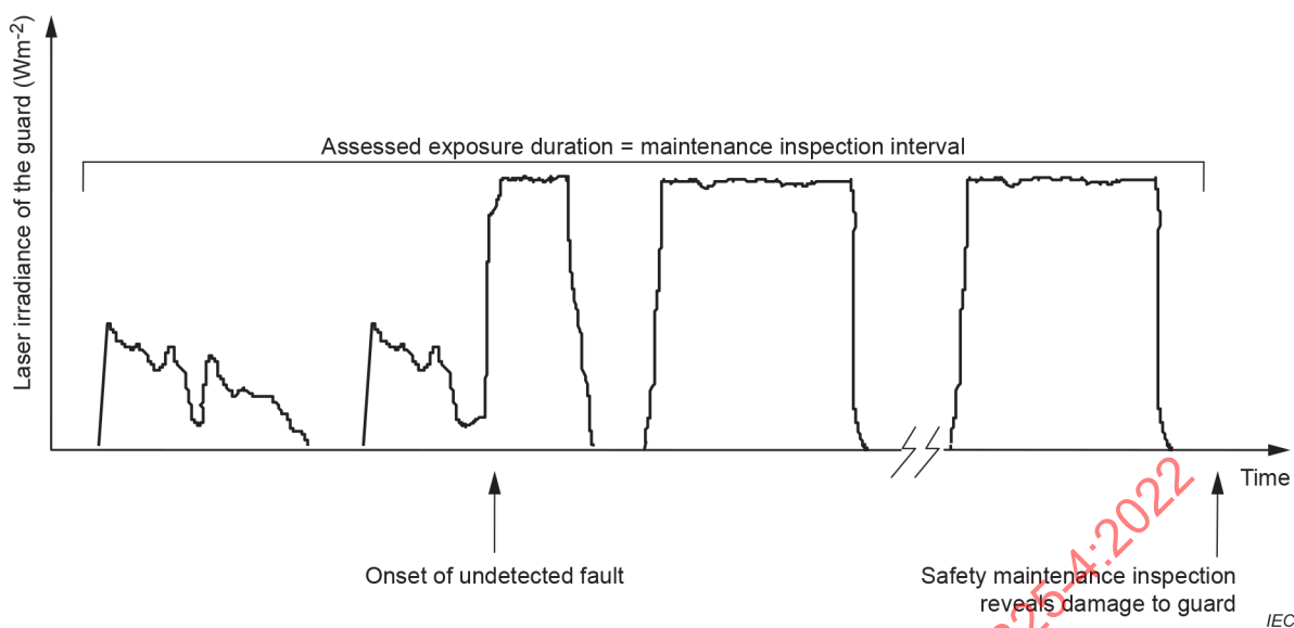
Figure B.7 – Assessed duration of exposure for a machine with no safety monitoring
