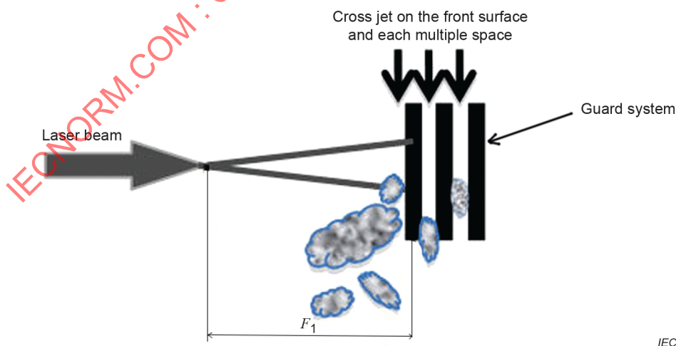
Figure D.2 – Simplified diagram of the ventilation for the guard under test
