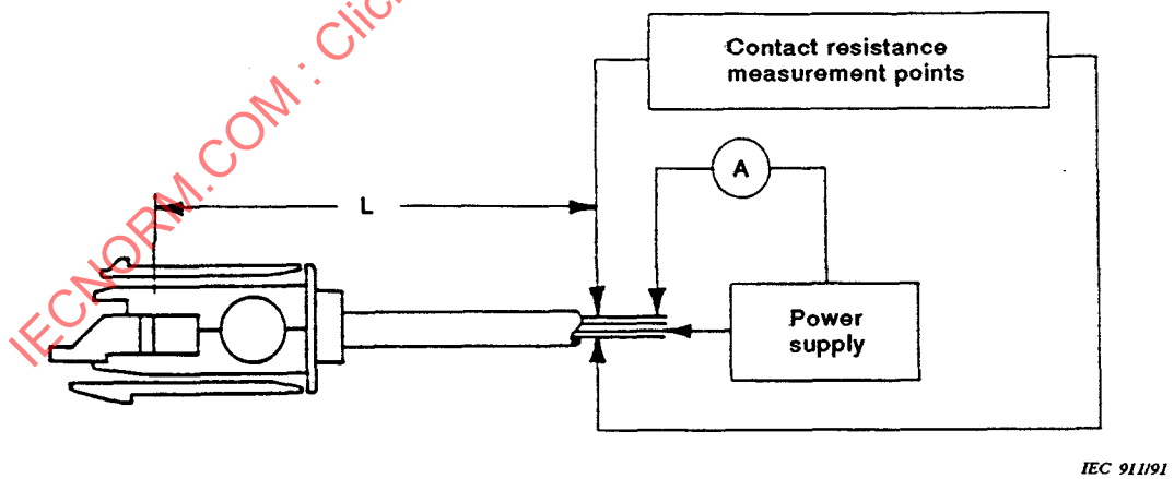
Figure 12 - Contact resistance measurement points, unmated
