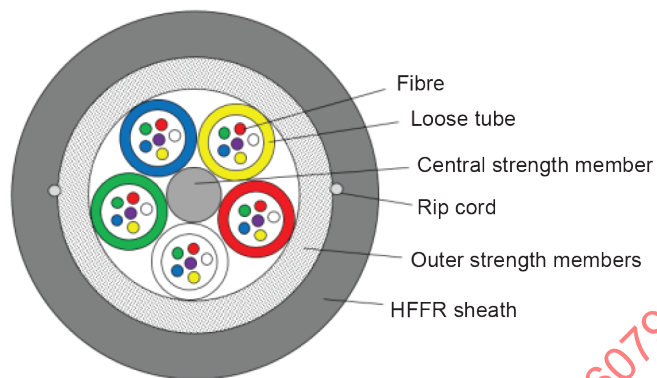
Figure A.1 – Example of a stranded universal indoor-outdoor cable design
