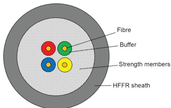
Figure A.3 – Mini-breakout universal indoor-outdoor cable design
