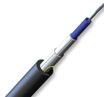
Figure A.2 – Example of an universal indoor-outdoor cable with a central tube design
