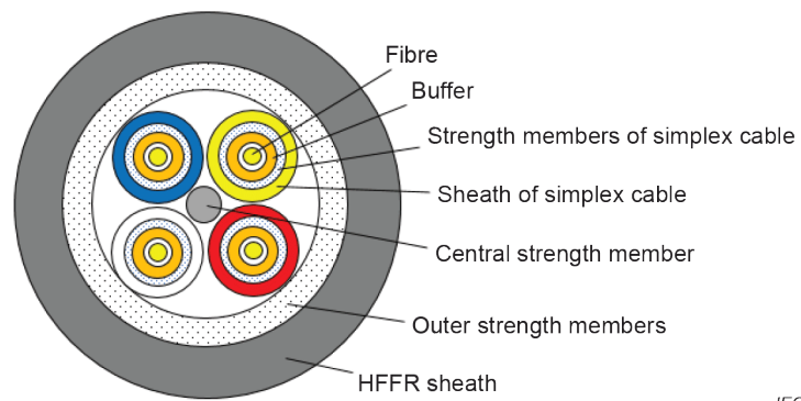
Figure A.4 – Breakout universal indoor-outdoor cable design
