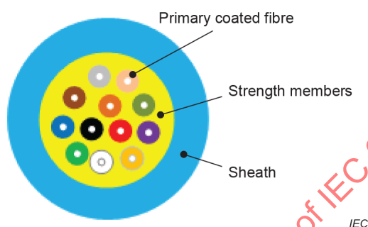
Figure B.1 – Example of a cross-section of a 12-fibre cable with single sheath
