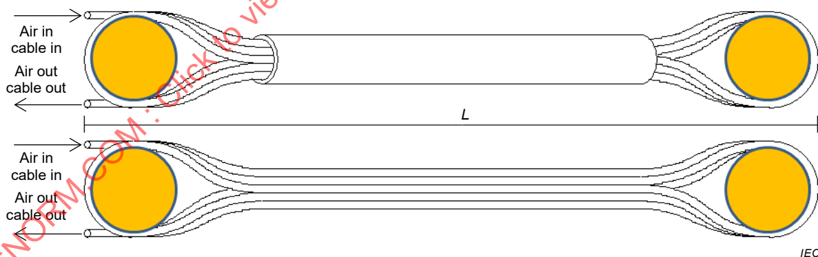
Figure 32a – Protected microduct
