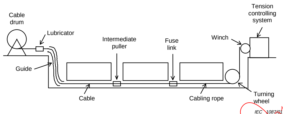
Figure A.2 – Optical fibre cabling in an underground duct
