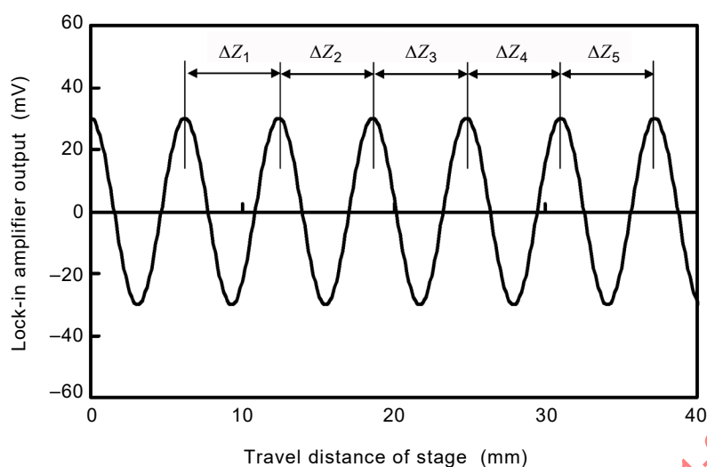
Figure 2 – Example of measurement profile by electromagnet
