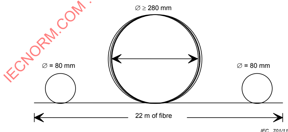
Figure 1 – Deployment configuration for cable cut-off wavelength, method A
