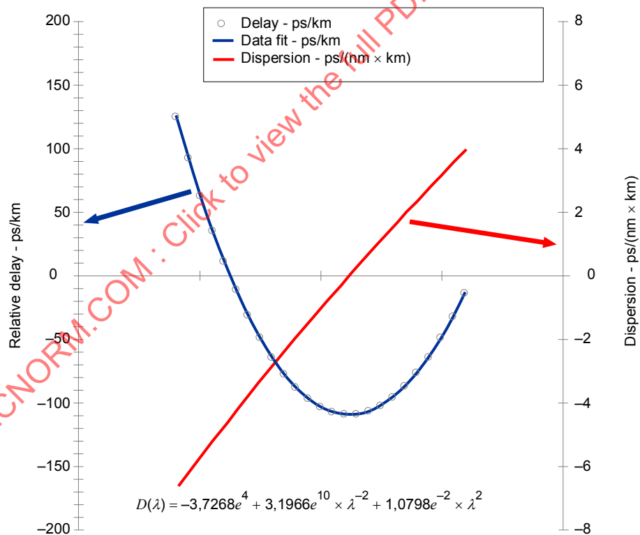
Figure A.2 – Typical delay and dispersion curves
