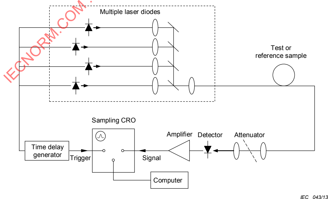
Figure B.2 – Block diagram, multiple laser diode system
