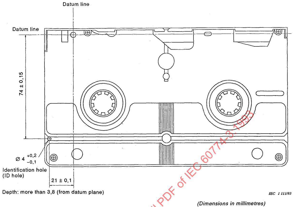
Figure 1 – Identification hole (ID hole) of cassette
