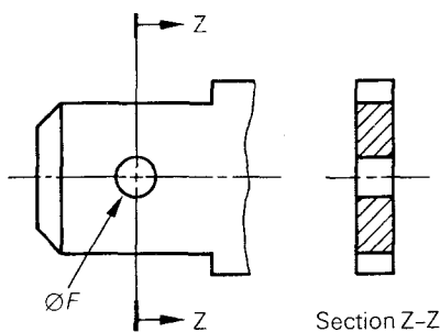
FIG. 3. — Dimensions of hole detents (see Figure 1, page 11).
