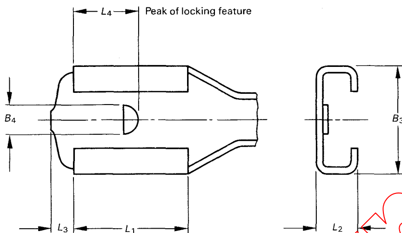
FIG. 4a. — Dimensions of female connectors, alternative design.
