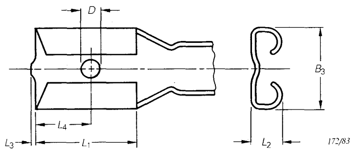
FIG. 4. — Dimensions of female connectors.
