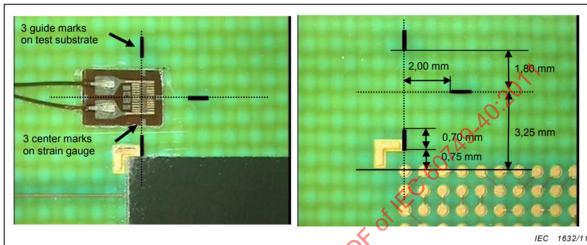
Figure B.2 – Example of Attaching Strain Gauge and Guide Mark Dimensions
