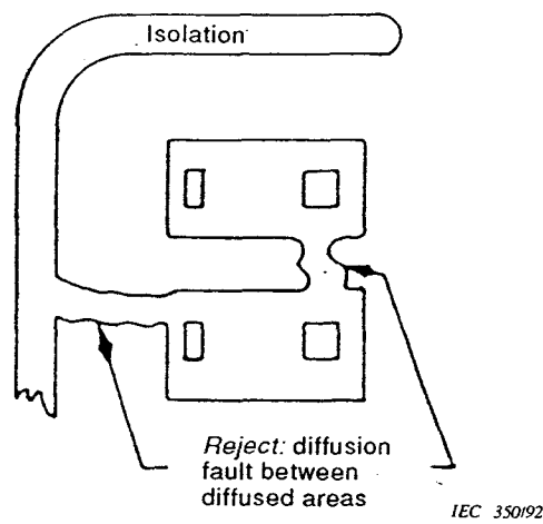
Figure 9 – Diffusion faults
