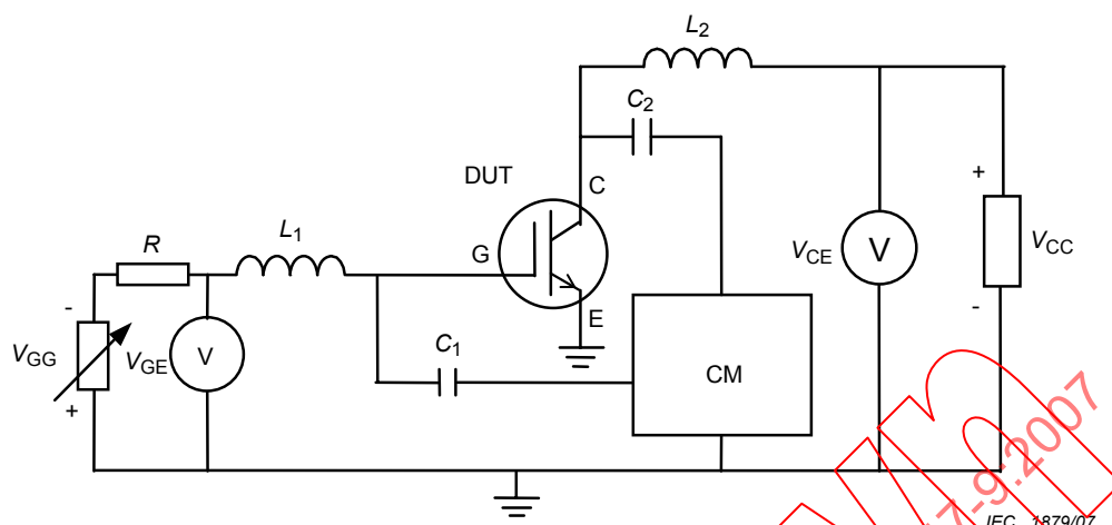
Figure 19 – Circuit for measuring the reverse transfer capacitance
