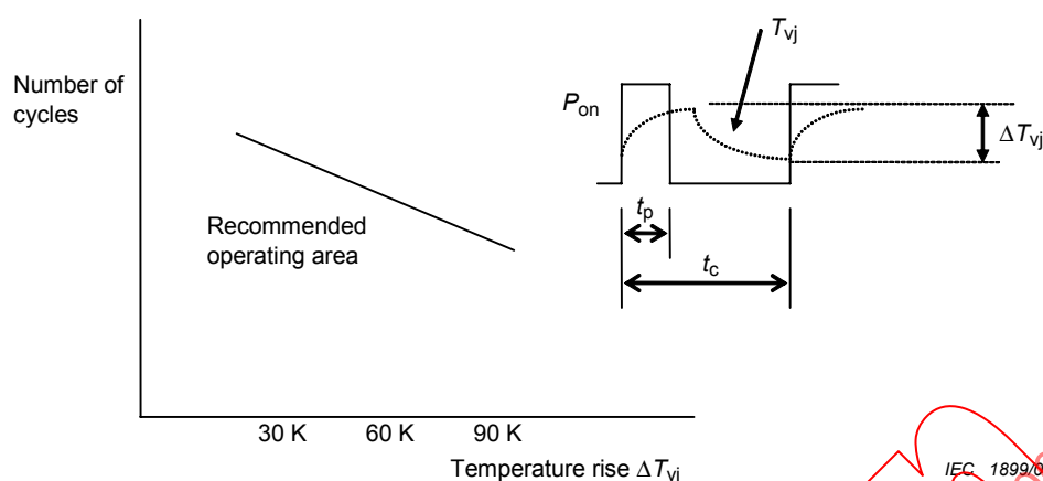
Figure 35 – Expected number of cycles versus temperature rise \Delta T_{vj}
