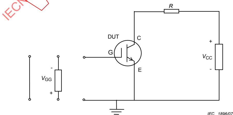
Figure 32 – Circuit for high-temperature blockings
