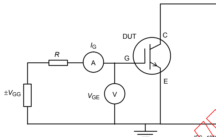
Figure 2 – Circuit for testing the gate-emitter voltage \pm V_{GE}
