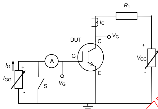
Figure 20 – Circuit for measuring the gate charge
