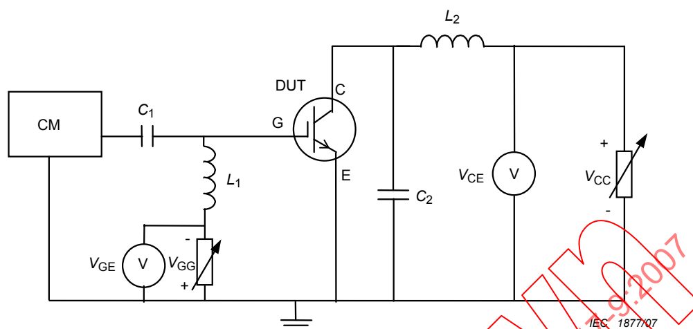
Figure 17 – Circuit for measuring the input capacitance
