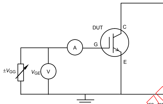
Figure 16 – Circuit for measuring the gate leakage current
