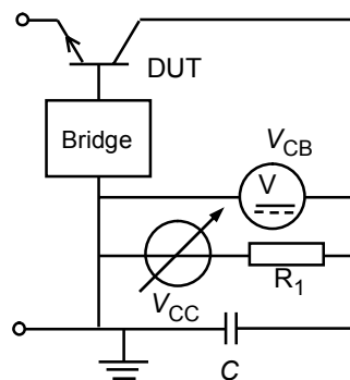
Figure 25b – Transistor with collector terminal connected to case
