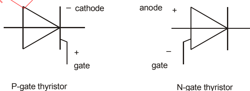
Figure 17 – Application of gate voltages for thyristors
