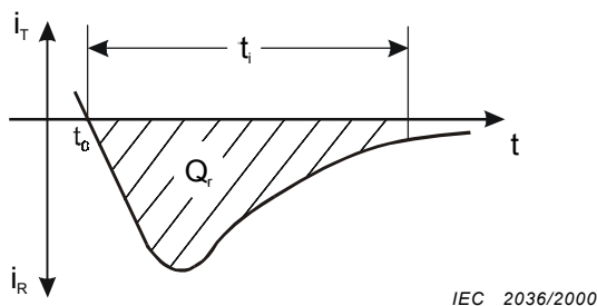
Figure 14 – Charge de recouvrement Q_r
