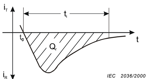
Figure 14 – Recovered charge Q_r
