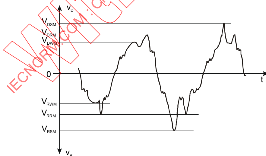
Figure 15 – Letter symbols for rated off-state reverse voltages
