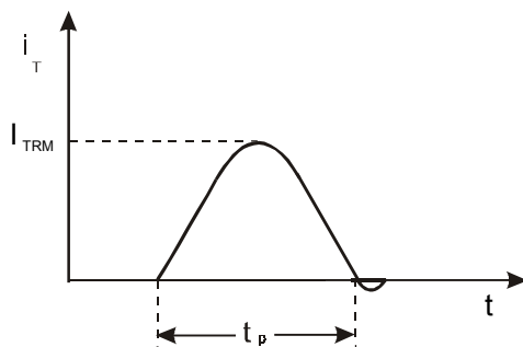
Figure 22b – Single sinusoidal on-state current pulse
