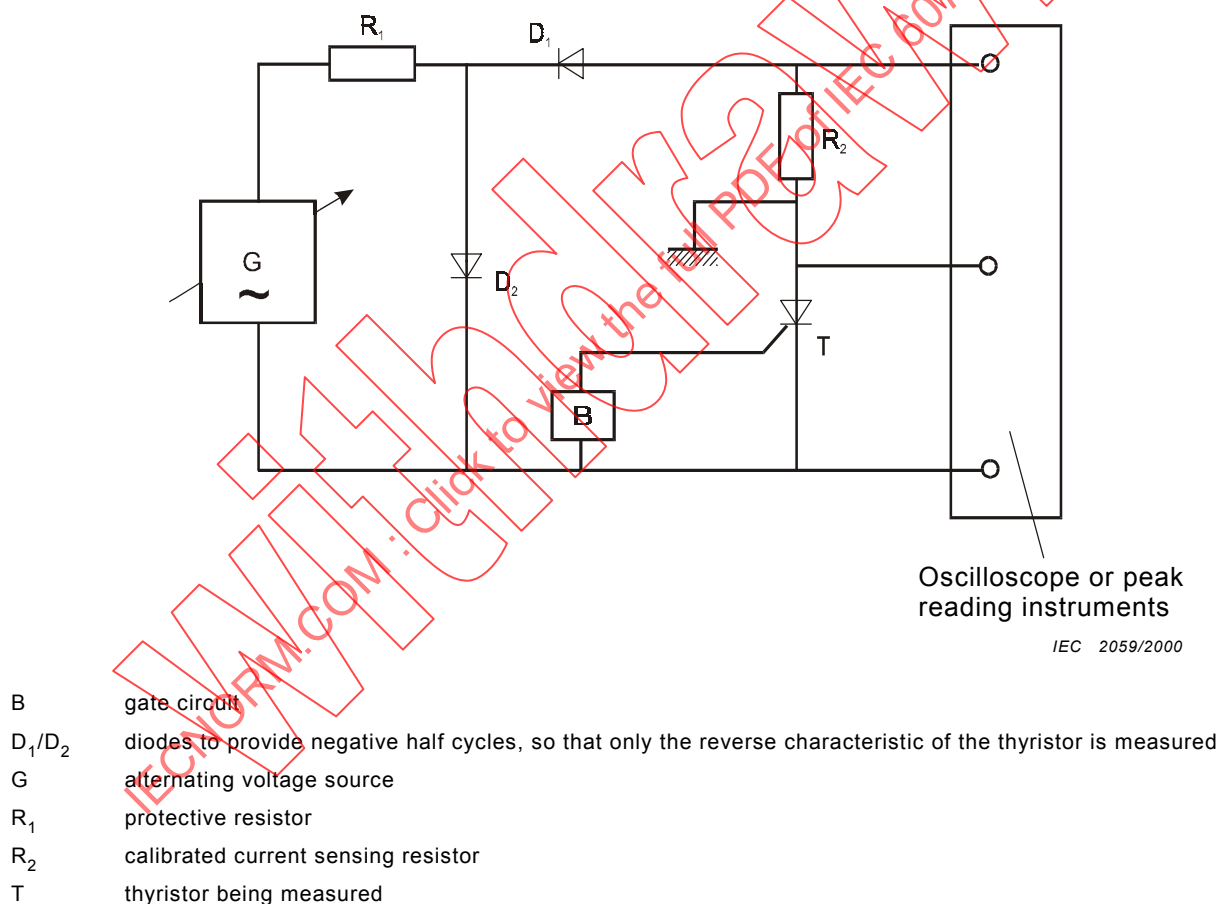
Figure 29 – Circuit diagram for measuring peak reverse current
