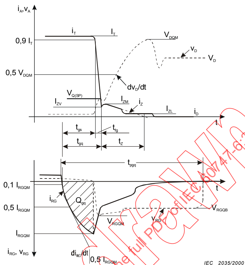
Figure 13 – Gate-controlled turn-off times
