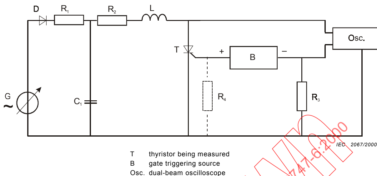
Figure 37 – Circuit diagram for measuring the gate controlled delay time and turn-on time
