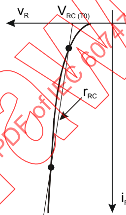
Figure 8b – Reverse-conducting characteristic
