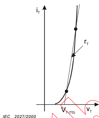
Figure 8a – On-state characteristic
