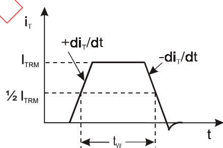
Figure 23a – Total energy loss E_p during a single trapezoidal on-state current pulse of duration t_w and amplitude I_{TRM}
