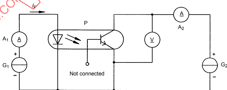
Figure 9 – DC measurement circuit
