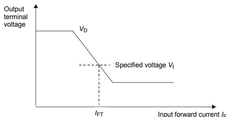
Figure 24 – Output terminal voltage versus input forward current
