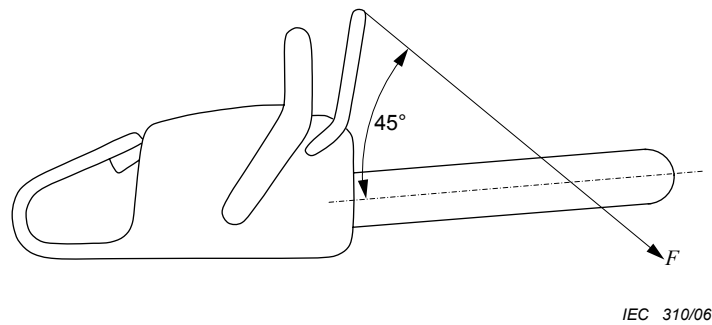
Figure 107 – Static test for release force
