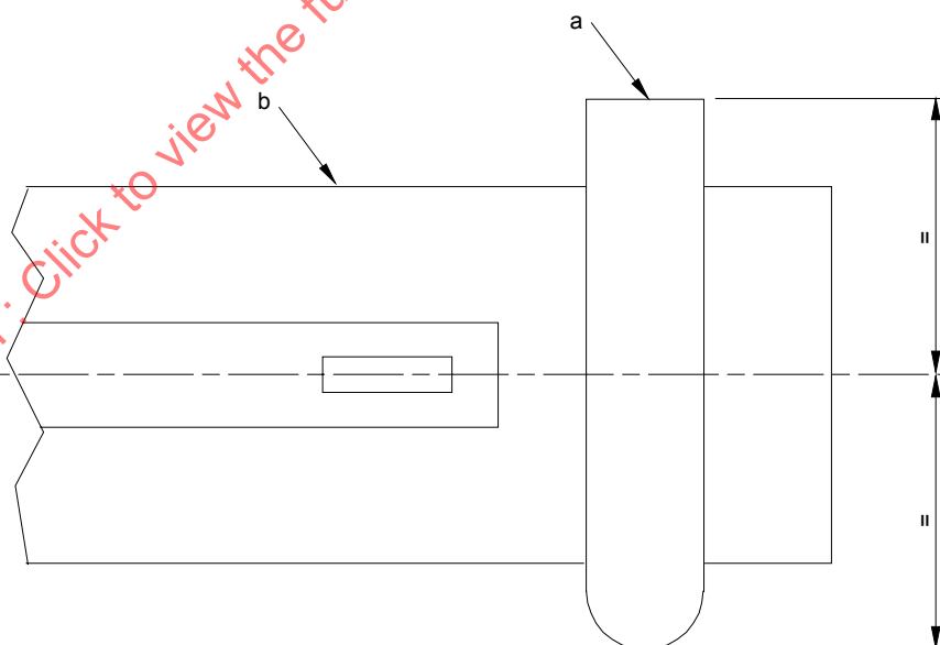
b) Side section showing position and direction of movement of test probe
