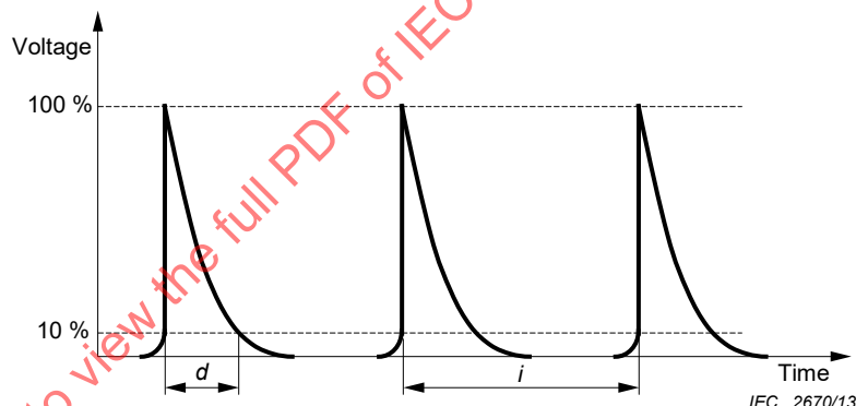
Figure 101 – Pulse spark generation
