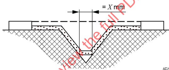
Figure B.2 – Wide groove
