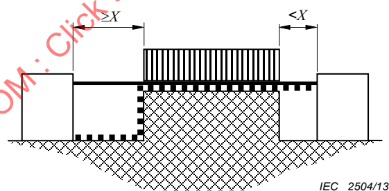
Figure B.6 – Uncemented joint with wide groove
