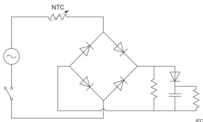
Figure J.1 – Generic test circuit for inrush-current limiting thermistor endurance test
