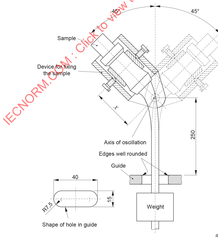
Figure 10 – Apparatus for flexing test
