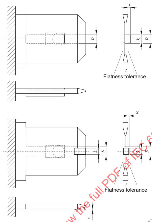
Figure 16 – Tabs for non-reversible connectors
