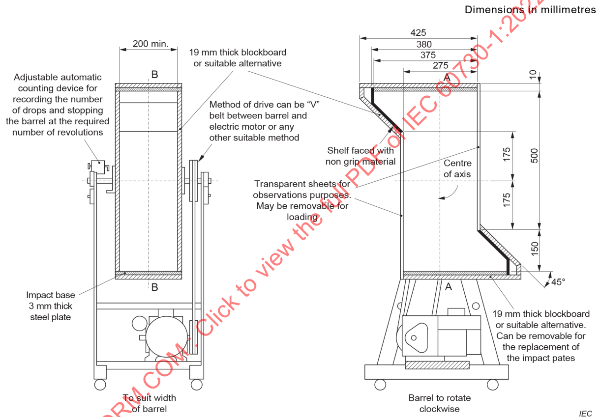
Figure 8 – Tumbling barrel
