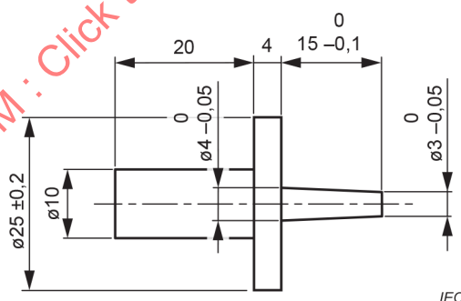
Figure 4 – Test pin probe 13 of IEC 61032:1997
