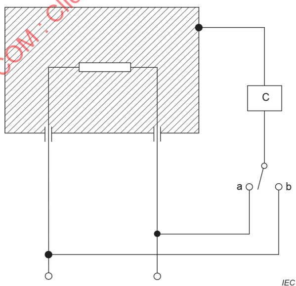
Figure 19 – Diagram for touch current measurement at operating temperature for single-phase connection of class II controls
