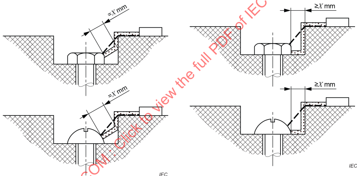
Figure B.8 – Diverging side walls
