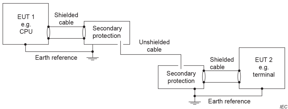
Figure N.2 – Example of secondary surge protection in buildings with separate common earth reference systems
