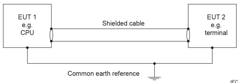
Figure N.1 – Example of surge protection by shielding in buildings with common earth reference systems
