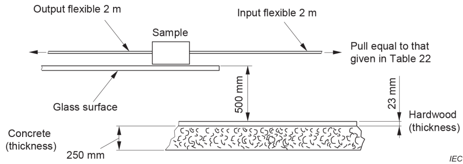
Figure 7 – Impact test for free-standing controls
