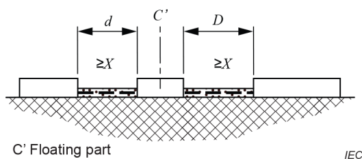
Figure B.11 – Conductive floating part
