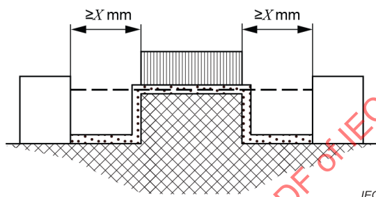
Figure B.5 – Uncemented joint with narrow groove
