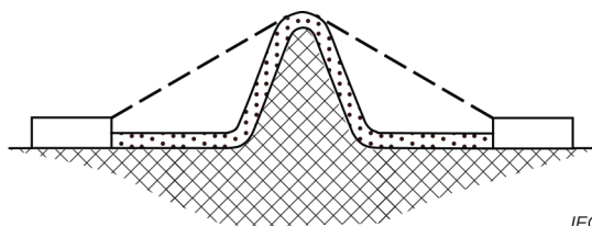
Figure B.3 – V-shaped groove
