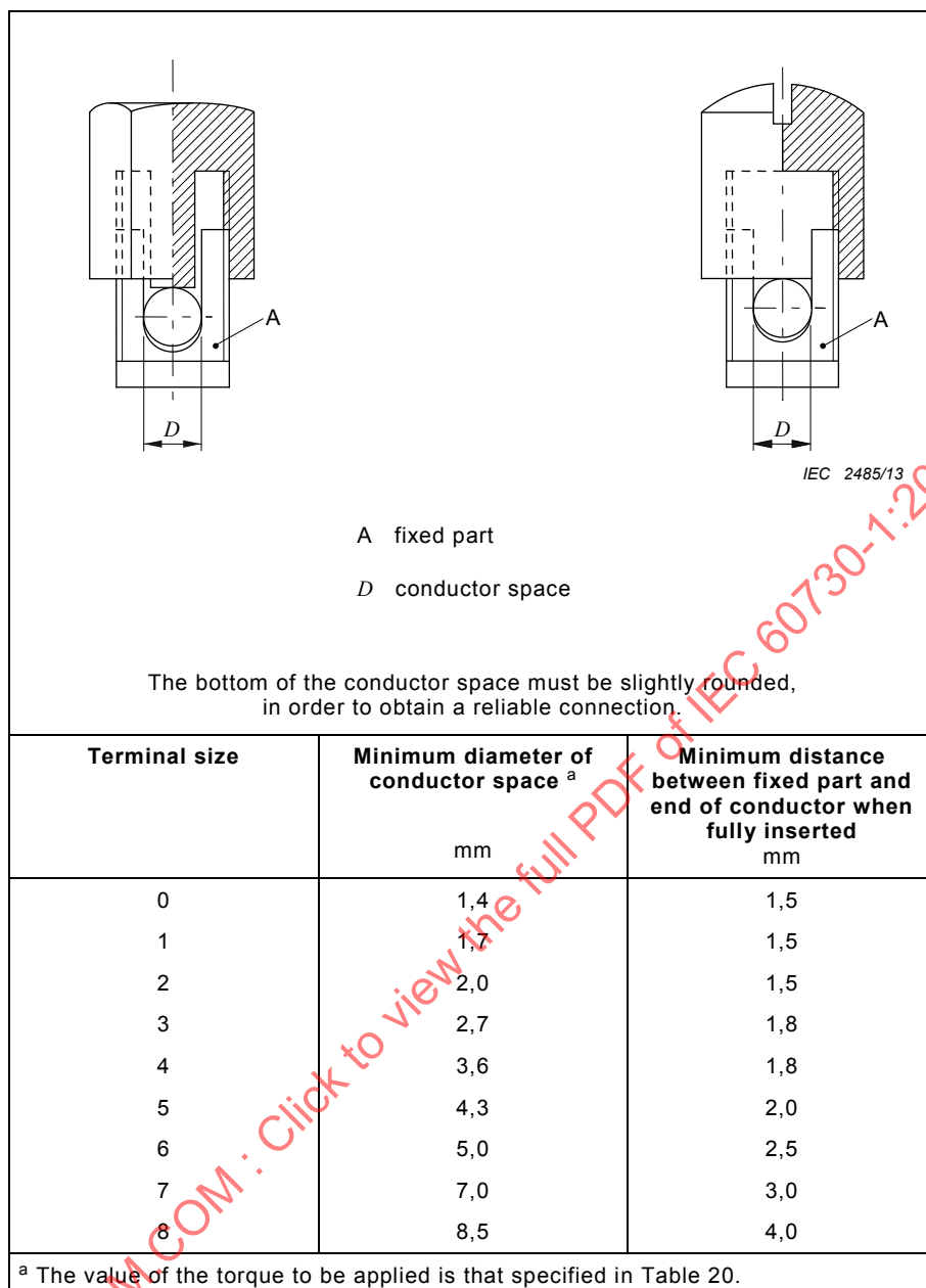
Figure 12 – Mantle terminals
