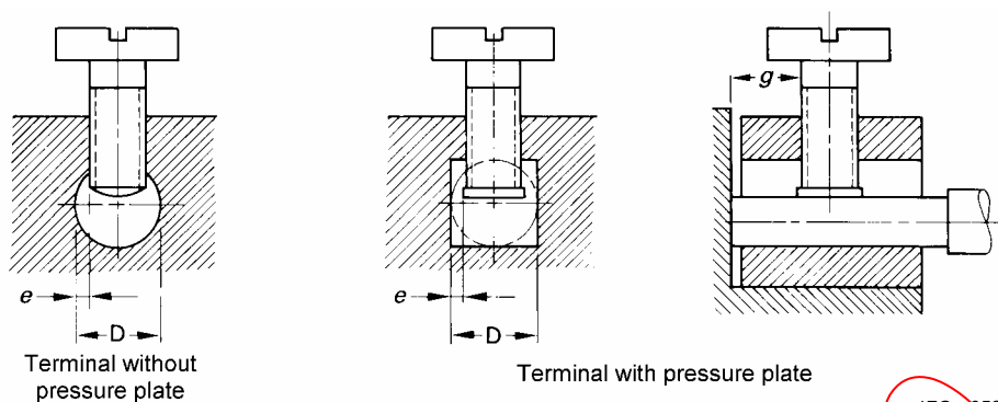
Figure 11 – Pillar terminals
