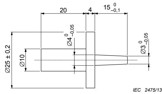
Figure 1 – Test pin
