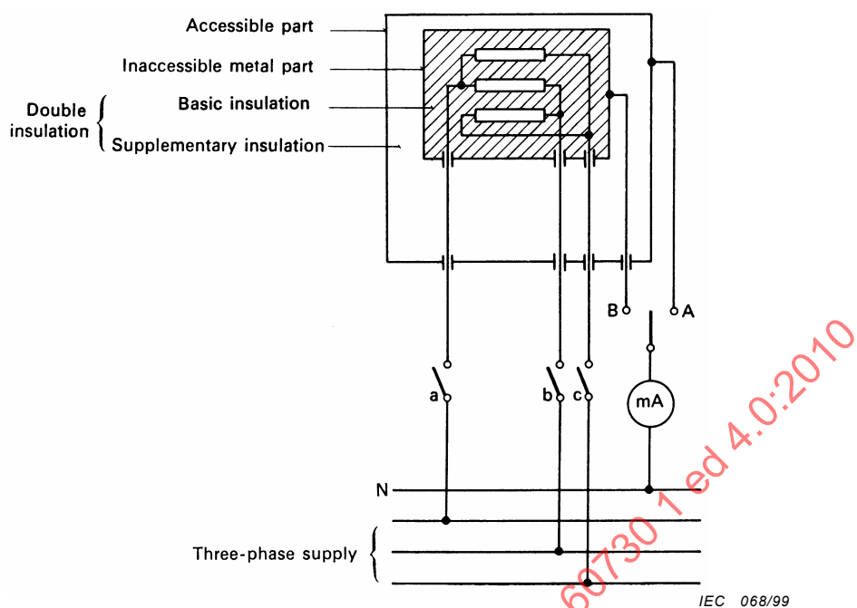
Figure 27 – Diagram for leakage current measurement at operating temperature for three-phase connection of class II controls
