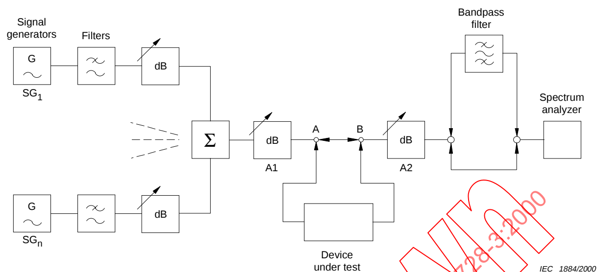
Figure 4 – Connection of test equipment for the measurement of non-linear distortion by composite beat
