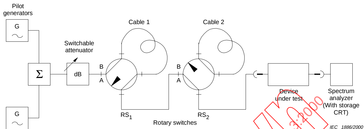
Figure 6 – Measurement of the AGC step response
