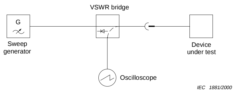
Figure 1 – Measurement of return loss
