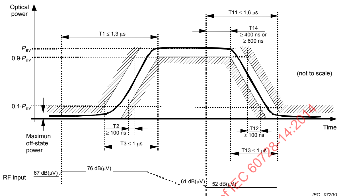
Figure 4 – R-ONU turn-on and turn-off diagram
