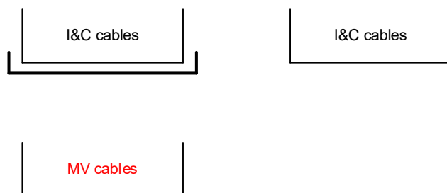
EMC protection for I&C cables – plate or cover at the bottom
