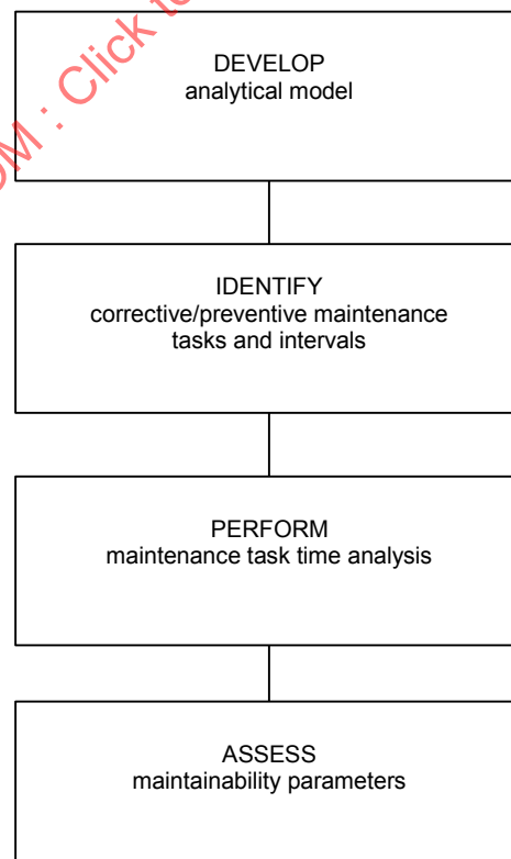
Figure 3 – Basic steps in maintainability prediction
