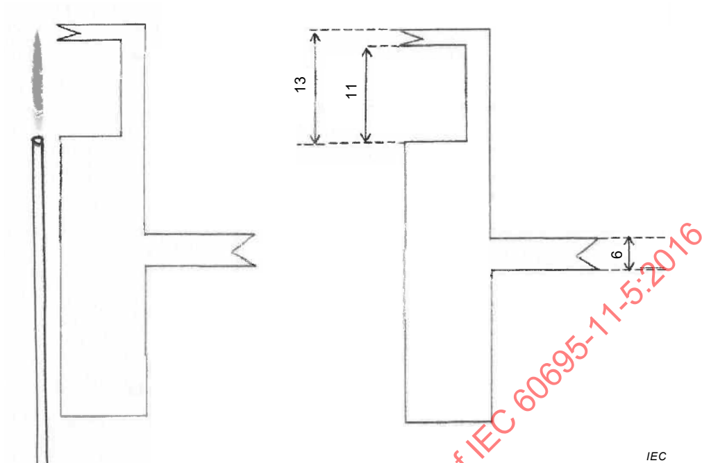
Figure A.3 – Gauge to measure flame height and the distance between burner and copper block (example)
