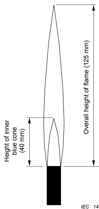
Figure 1 – Flame dimensions
