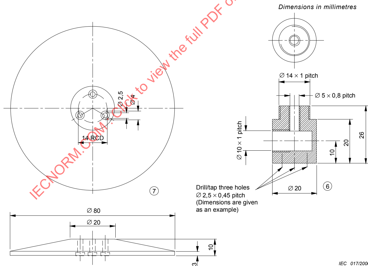
Figure B.3 – Burner details – Gas supply tube and gas jet
