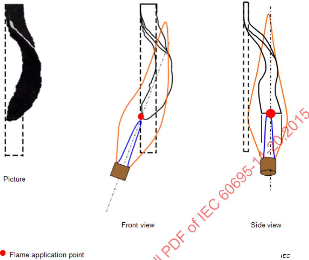
Figure A.2a) – Flame application point for a twisted specimen
