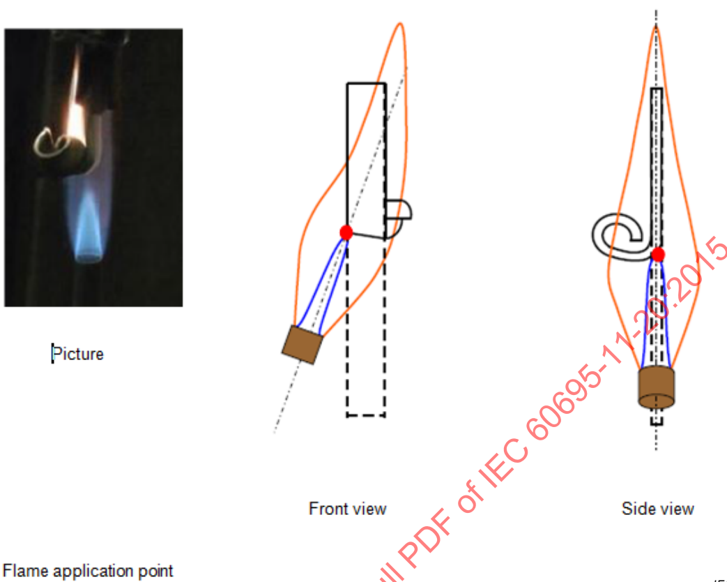
Figure A.3 – Flame application point for a curled specimen
