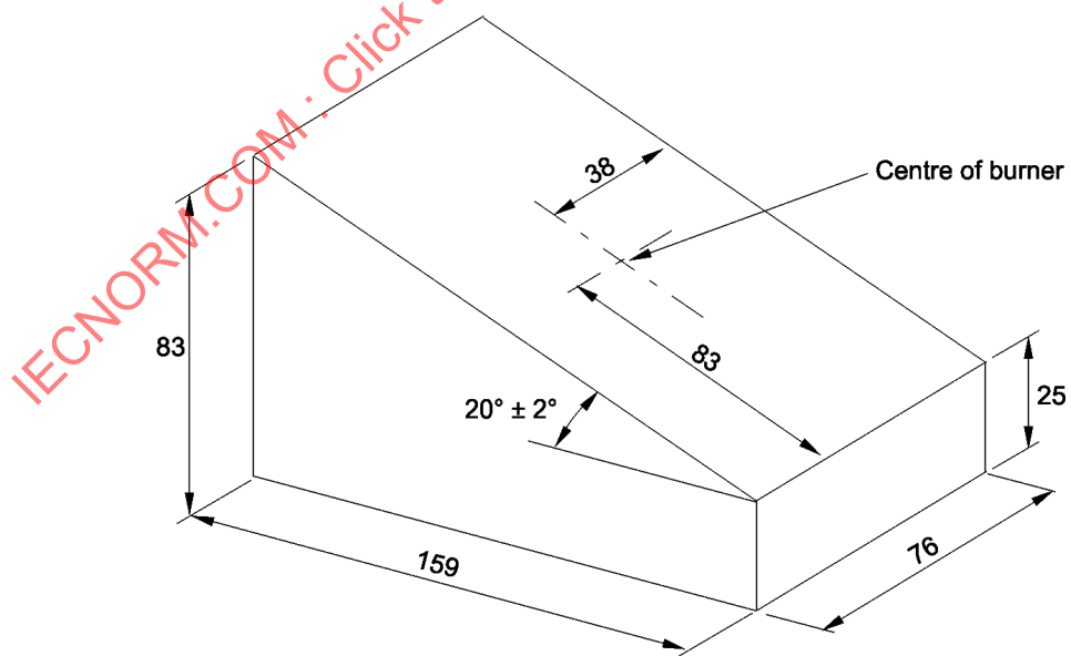
Figure 2 – Horizontal burning test for plates
